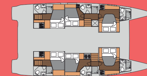
6 CABINS VERSION
