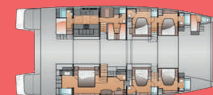
VIP + 4 GUESTS + CREW QUARTER
