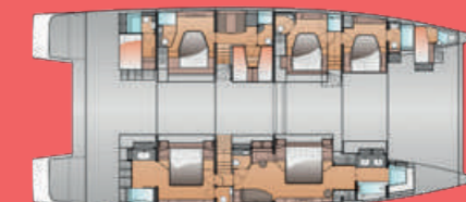
MAESTRO + VIP + 3 GUESTS + CREW QUARTER
